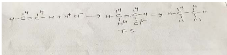
Addition of Acid to Ethene molecule
